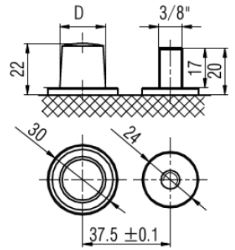
DT-3/8 Terminal
